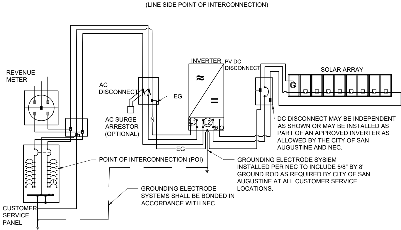
FIGURE 3 TYPICAL PHOTOVOLTAIC (PV) SYSTEM 120/240-VOLT SINGLE-PHASE THREE-WIRE DIAGRAM
